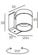
WLB083-1/1 x 4W
