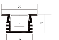
MLL2212R
