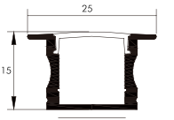
MLL2415R
