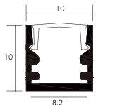
MLL1010
