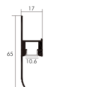
MLL1765
