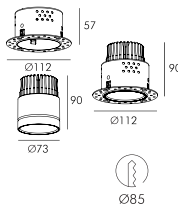
SL74346/12W
