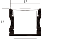
MLL1715
