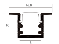
MLL1710R
